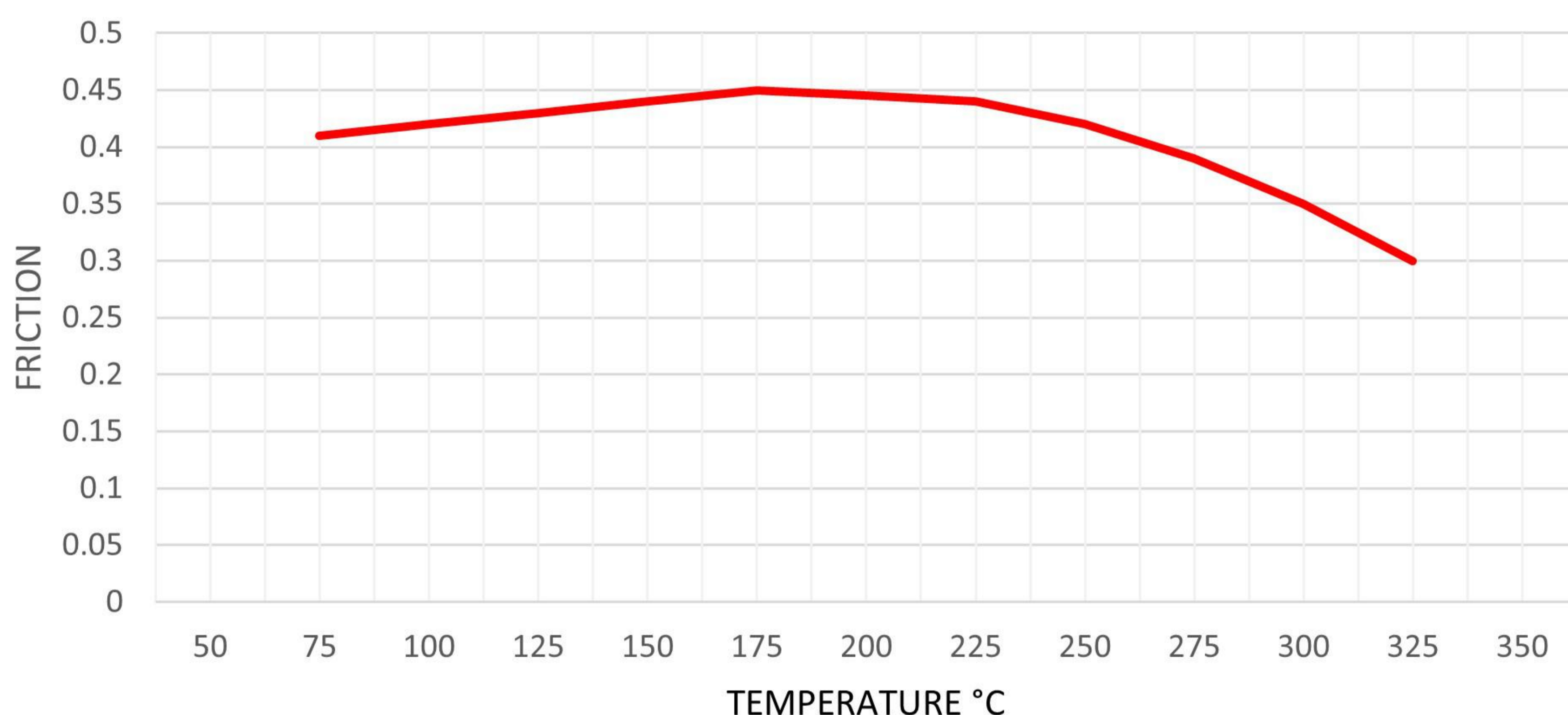
FRICITION/TEMPERATURE
